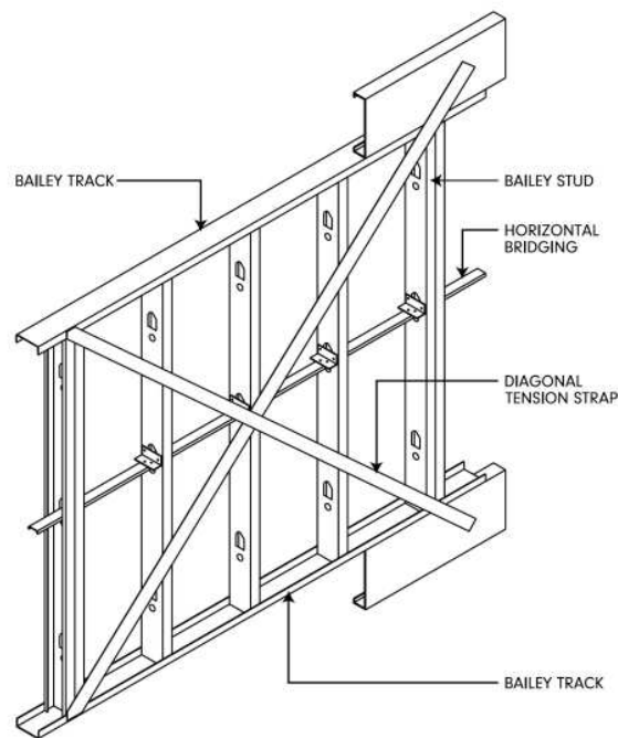
35 – Diagonal Tension Straps One Side
