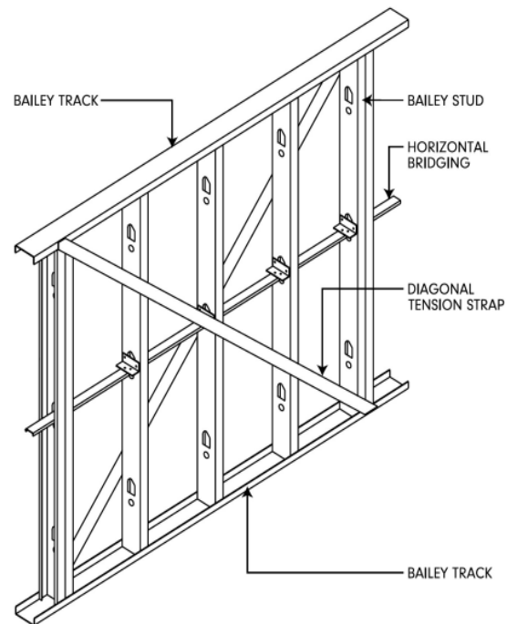
36 – Diagonal Tension Straps Both Sides
