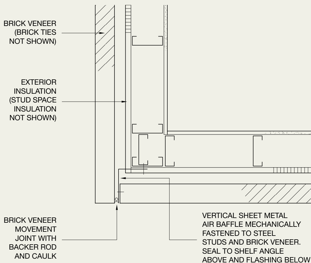
Figure 9b: Corner air baffle to reduce horizontal air flow cavity.
