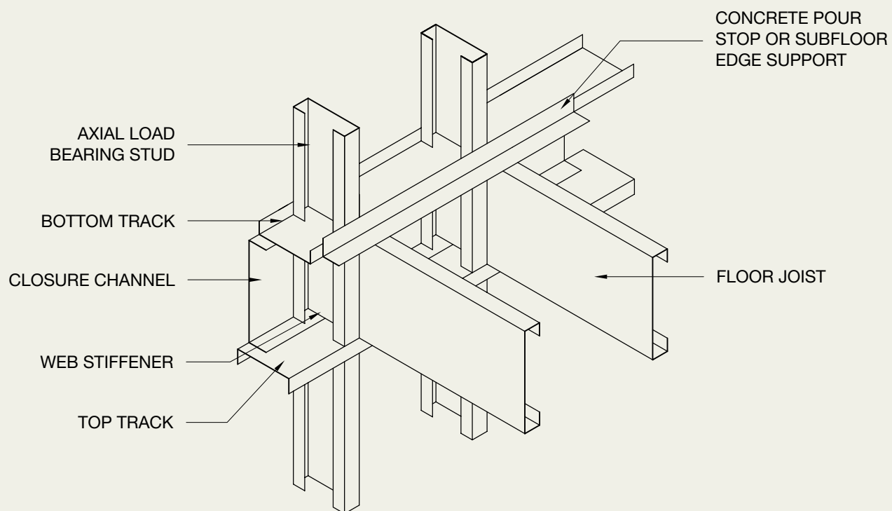
Figure 4: Typical platform framing detail.
