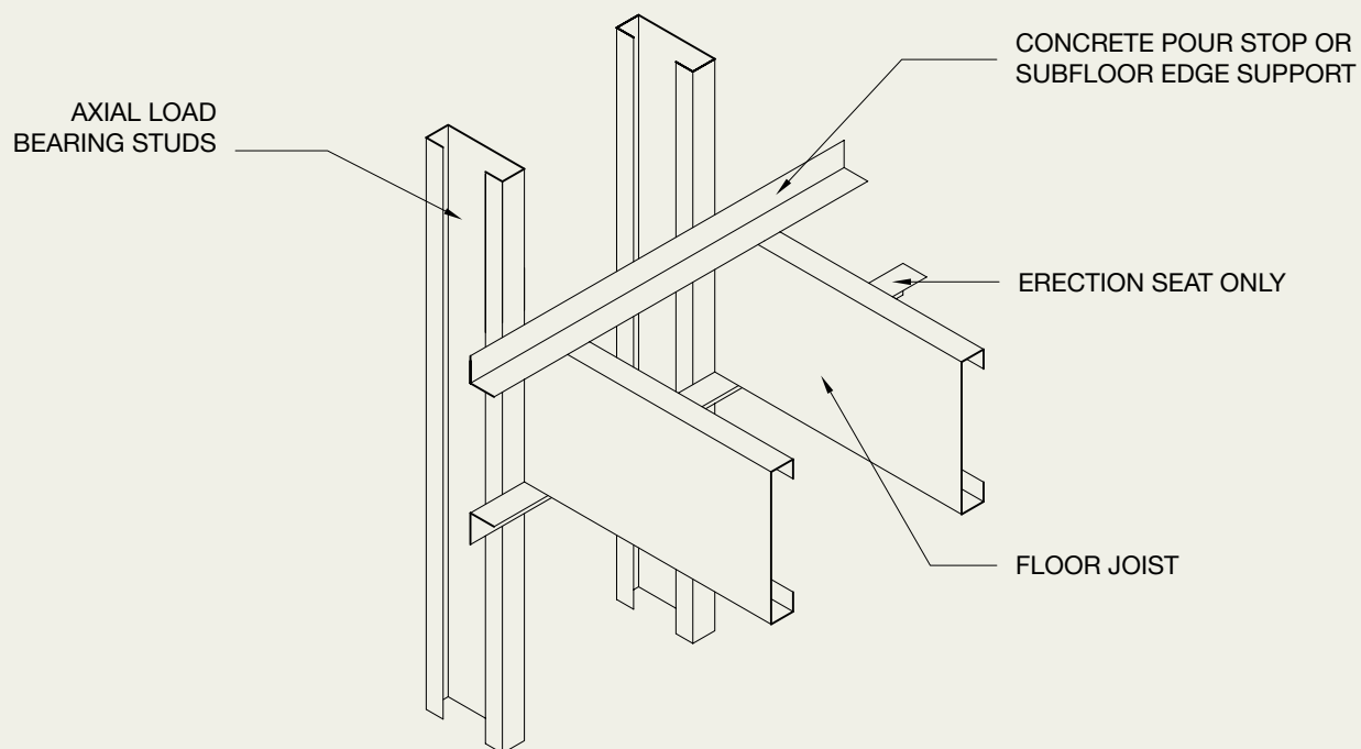
Figure 5a: Typical balloon framing detail.
